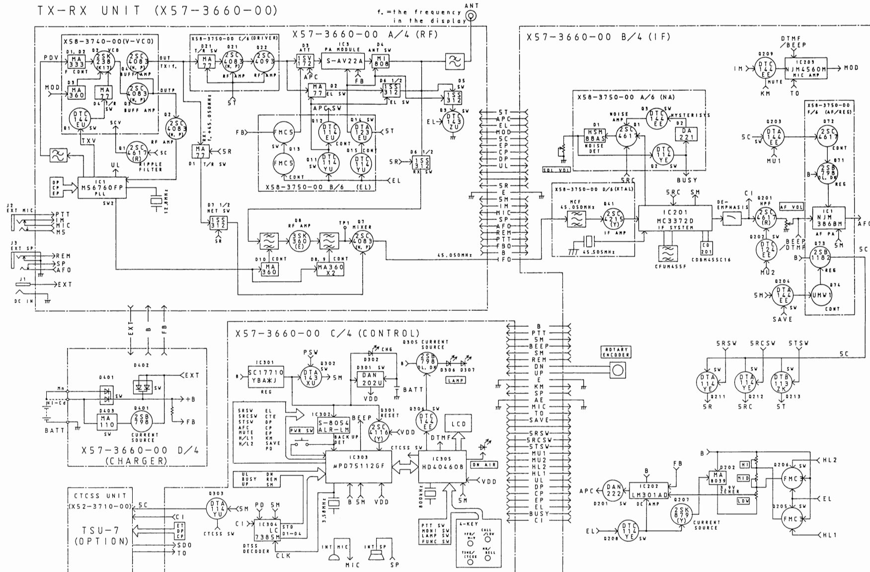
TH-K27 BLOCK DIAGRAM
