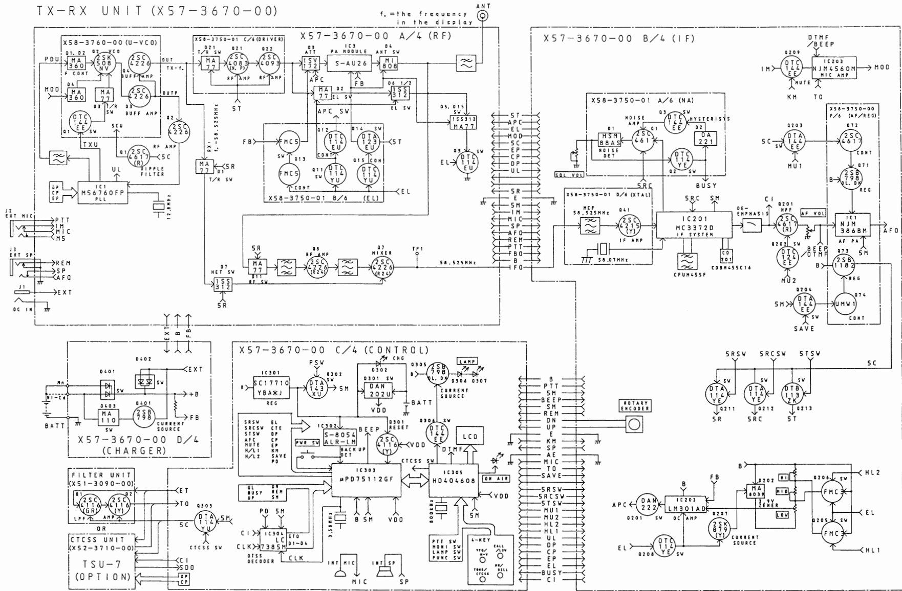
TH-K47 BLOCK DIAGRAM
