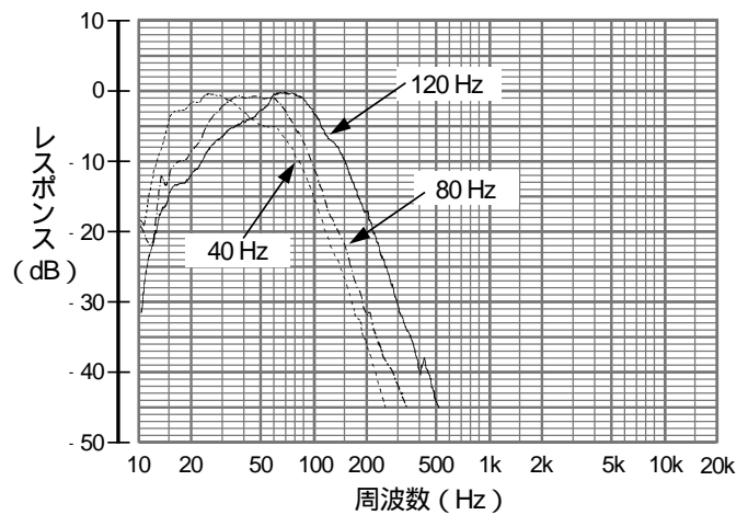
CUT OFF FREQUENCY 特性
